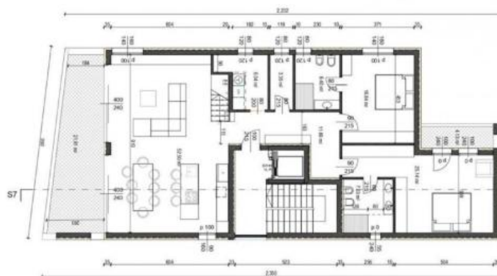
PENTHOUSE 2. KAT
